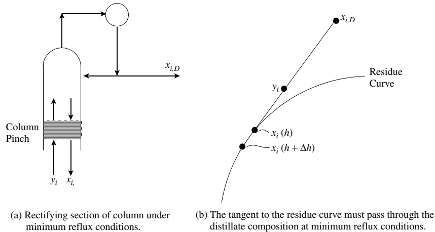
Figure 12.14 The minimum reflux condition can be identified from the tangent to the residue curve.
