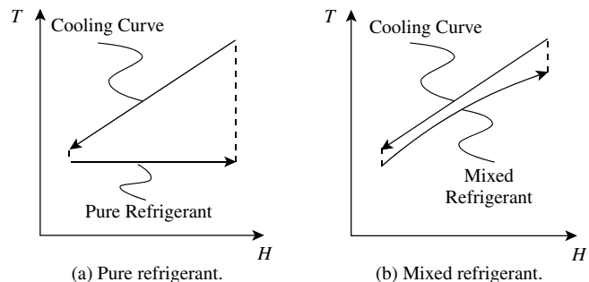
Figure 24.42 Pure and mixed refrigerants.
