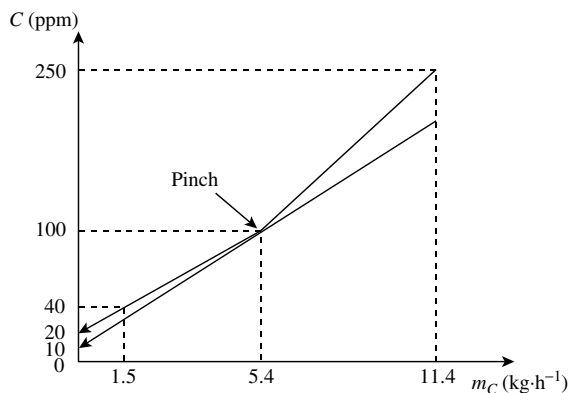
Figure 26.40 Targeting for a fixed outlet concentration of 10 ppm in Example 26.4.
