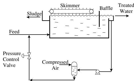
(b) Dissolved air flotation (DAF).
