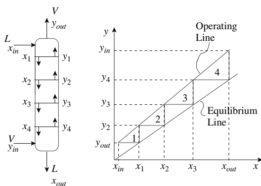
Figure 10.3 Equilibrium countercurrent stage operation for absorbers.
