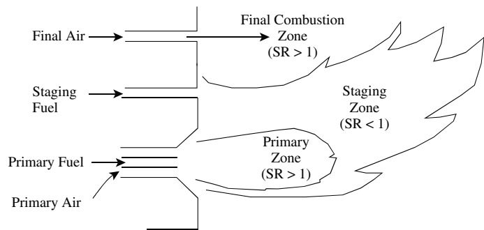
(b) Fuel staging.
