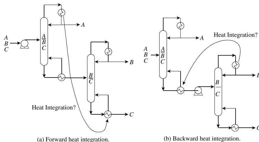
Figure 21.8 Heat integration of a sequence of two simple distillation columns. (From Smith R and Linnhoff B, 1988, Trans IChemE, ChERD , 66 : 195, reproduced by permission of the Institution of Chemical Engineers.)
