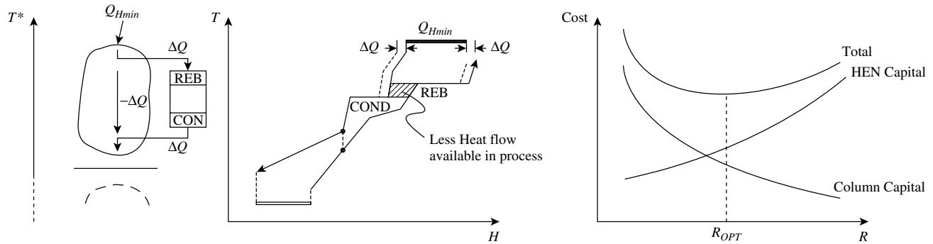
Figure 21.7 The capital/capital trade-off for an appropriately integrated distillation column. (From Smith R and Linnhoff B, 1988, Trans IChemE ChERD , 66 : 195, reproduced by permission of the Institution of Chemical Engineers.)
