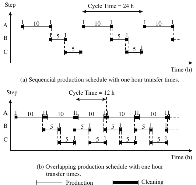
Figure 14.20 Transfer times extend the cycle times.
