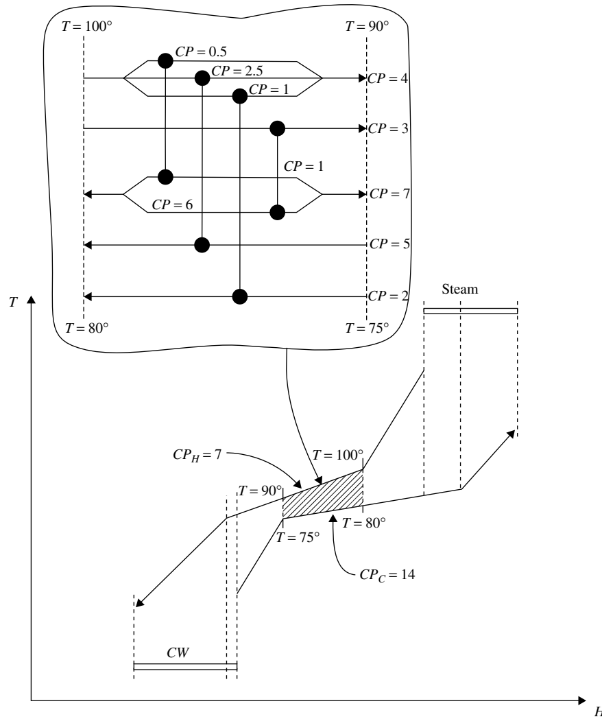
Figure F.1 Within each enthalpy interval it is possible to design a network in (S - 1) matches. (From Ahmad S and Smith R (1989) Targets and Design for Minimum Number of Shells in Heat Exchanger Networks, ICHEME, ChERD , 67 : 481, reproduced by permission of the Institution of Chemical Engineers.)
