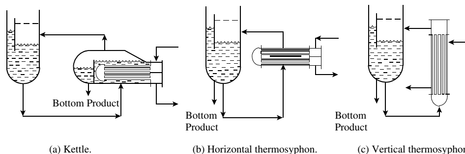
Figure 15.13 Reboiler designs.
