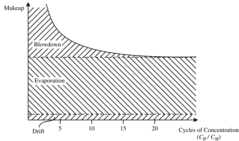
Figure 24.3 Relationship between makeup water and blowdown for cooling towers.
