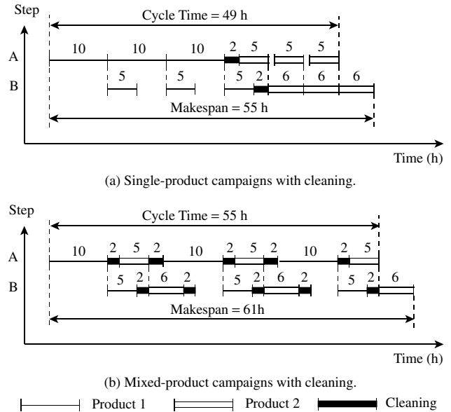
Figure 14.19 Cleaning between product changes extends the cycle times.
