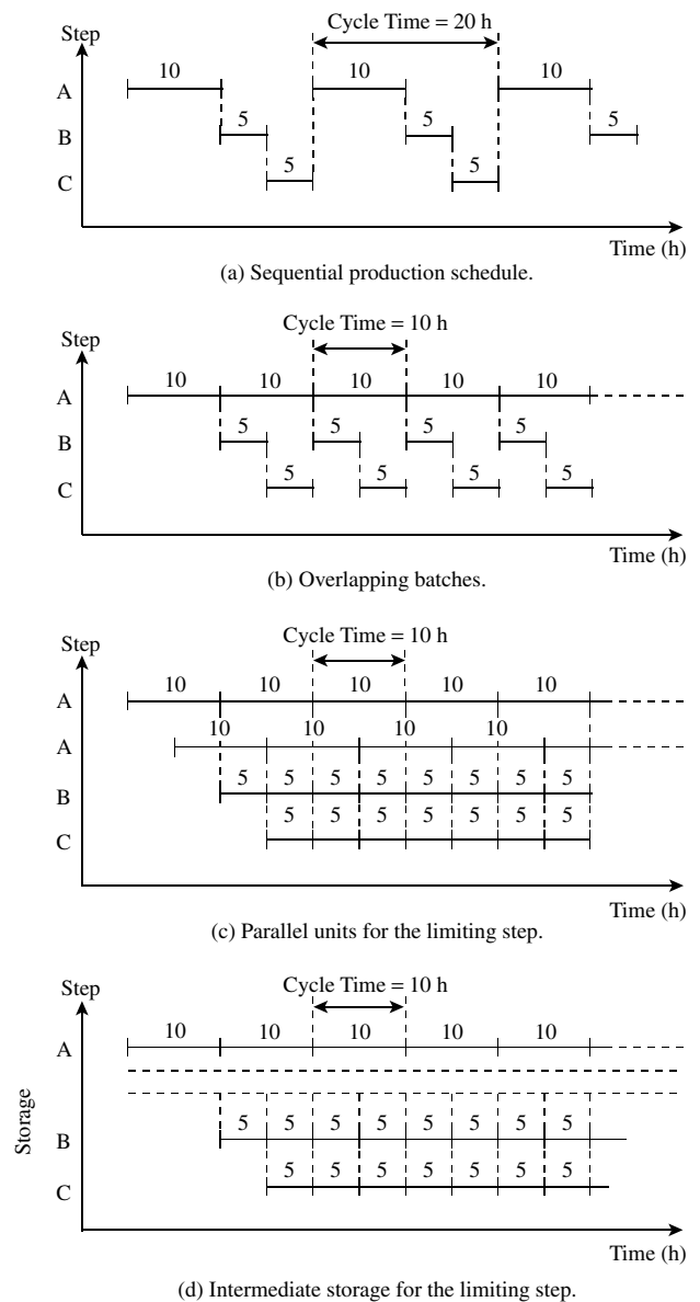
Figure 14.16 Production schedules for a three-step process.
