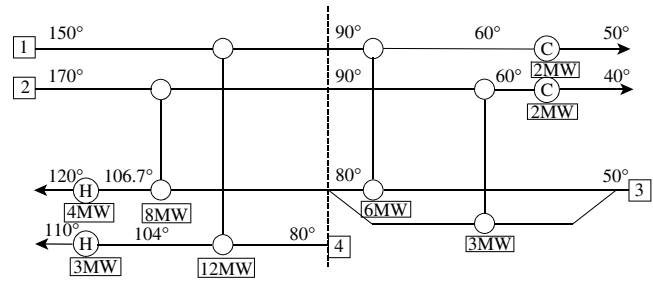
(a) The completed design.
