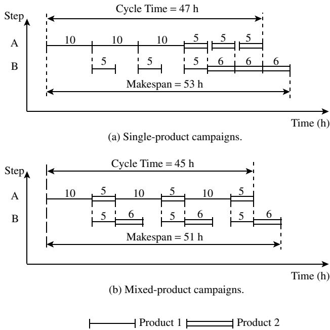
Figure 14.18 Single versus mixed-product campaigns for three batches each of two products.
