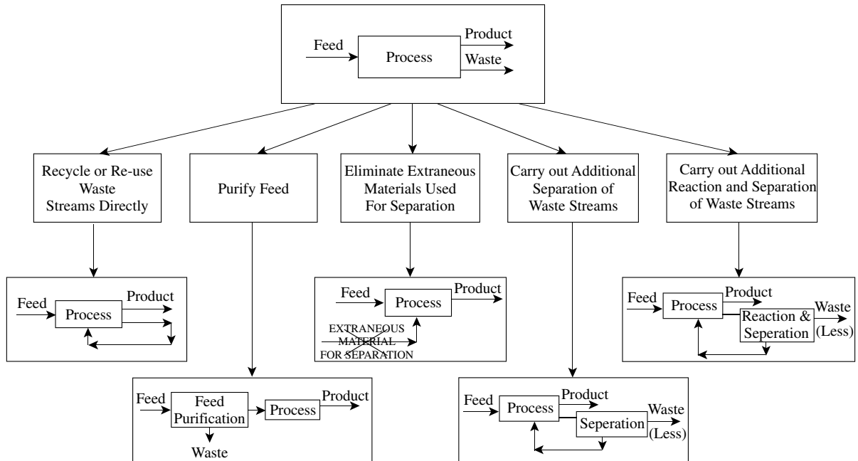
Figure 28.2 Waste minimization in separation and recycle systems.
