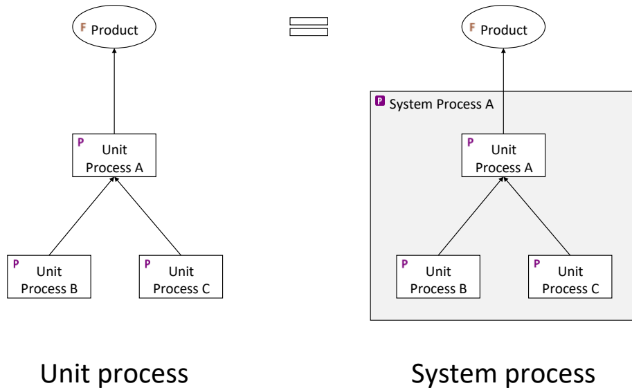
Figure 4.1: Unit and system processes
