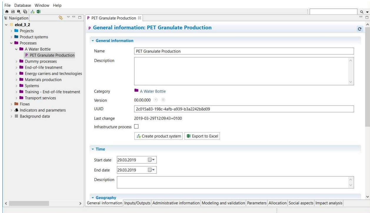
Figure 4.5: New Process in the Navigation and Editor window
