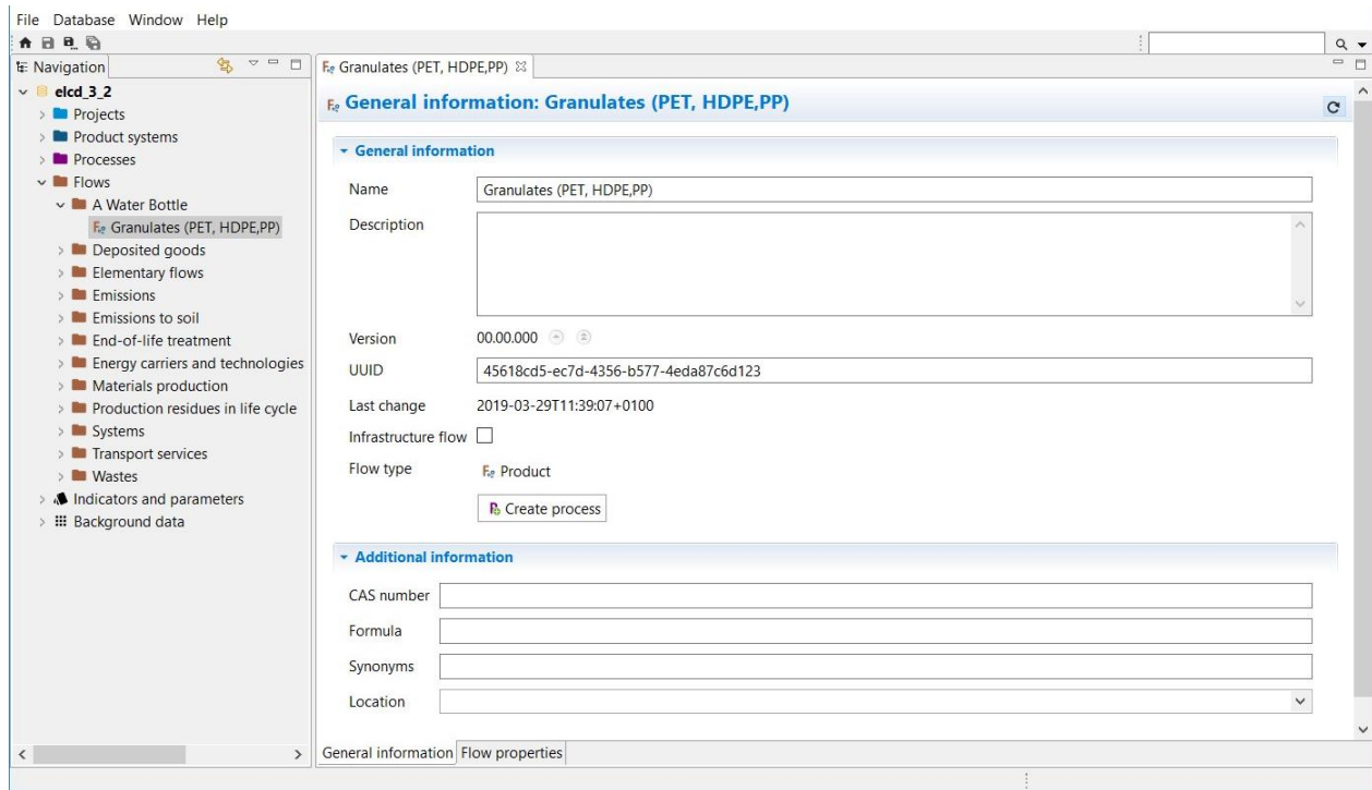
Figure 3.4: New flow in the Navigation and Editor window
