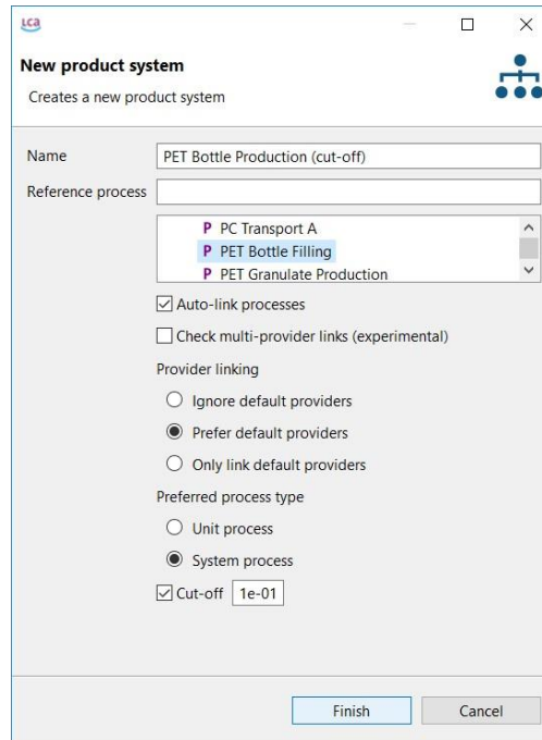
Figure 5.10: Create the product system PET BOTTLE PRODUCTION (CUT-OFF)
