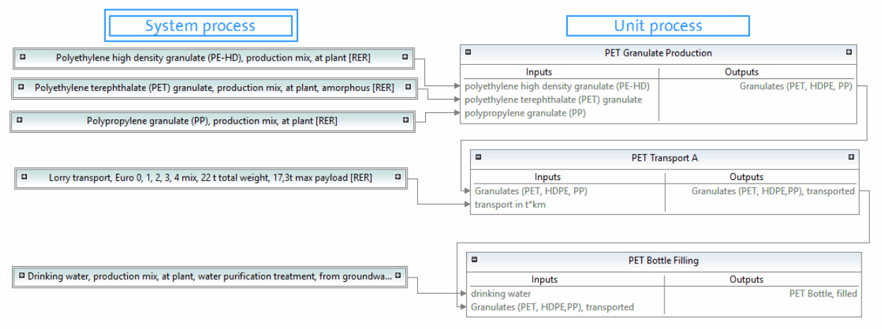
Figure 5.3: Model graph of the product system PET BOTTLE PRODUCTION
