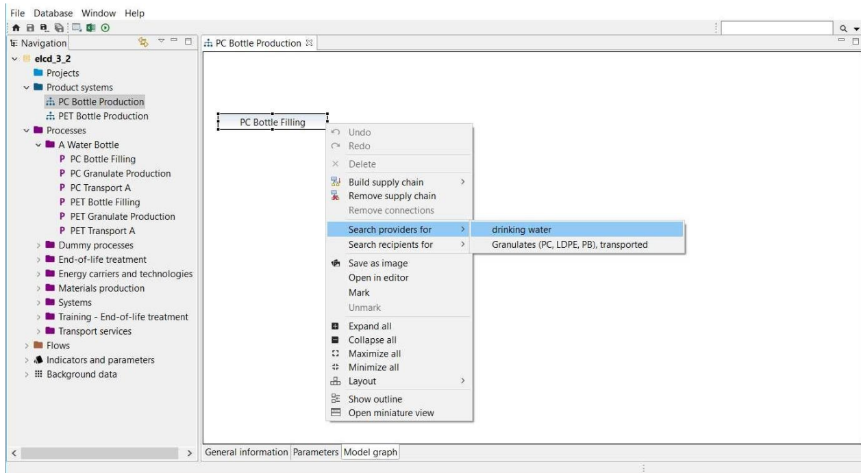
Figure 5.5: Create the product system PC BOTTLE PRODUCTION
