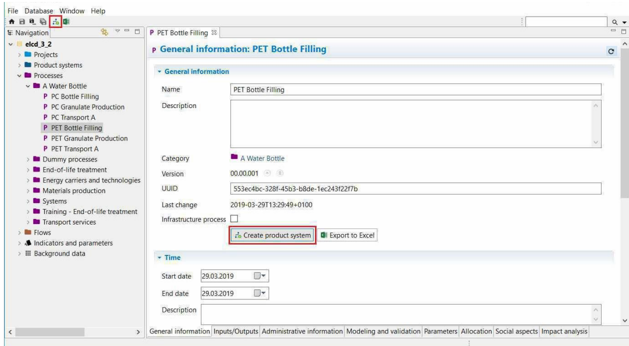
Figure 5.1: Create a product system in the process editor
